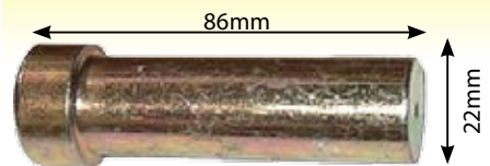
Drop In Pin - 2 Pin Type Push Back
