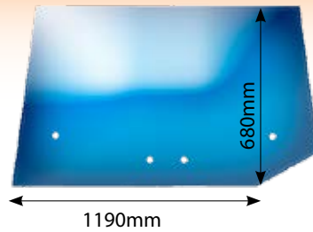
4230 Glass Case 3230 4210 4220 4230 4240 Upper Rear LP Series Cab - 6 Hole
