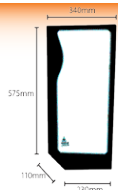
52453 Right Hand Glass Lower Front Case MXM120 140 155 175 190 M100 M115 M135 M160 8160 8260 8360 8560 OE Ref: 82001924
