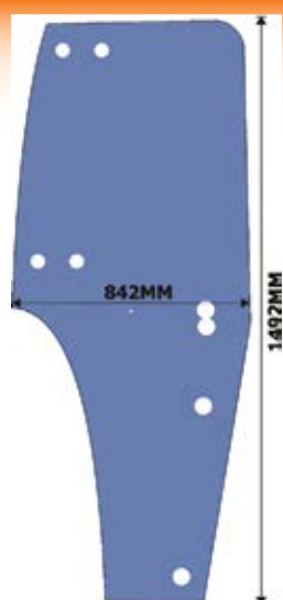
41077 Glass Door RH - 7 Hole MXM120-MXM190 JXU OE Ref: 82019225
