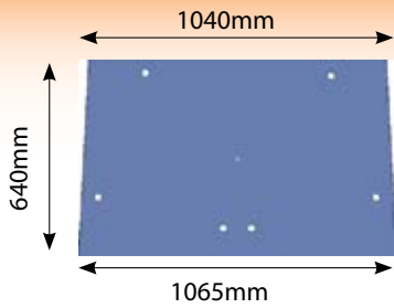
2223 Glass Ford AP IHC Super Deluxe Top Rear Glass 6 Hole Glass 584 684 784 884 385 485 685 785 885 585 484 OE Ref: 3125412R1
