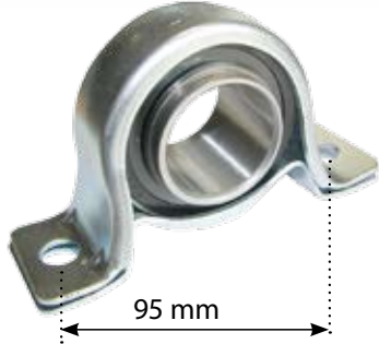
Shaft Drive Carrier & Bearing Kit IHC 4WD Bearing ID 32mm
