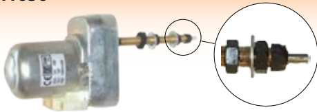
Wiper Motor 12 Volt 120 Straight Single Spin Shaft Length 99mm
