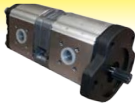
52406 Hydraulic Pump Tandem Case CS78 CS86 CS94 Bosch OE Ref: 0510765351
