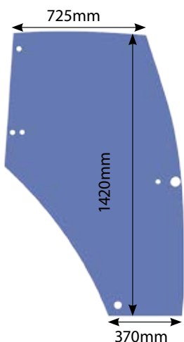
52095 Glass Case CX MX McCormick Door Right Hand
