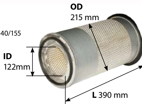
402819 Case Mxm130/140/155 Inner Air Filter
