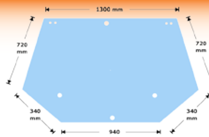
52453 Right Hand Glass Lower Front Case MXM120 140 155 175 190 M100 M115 M135 M160 8160 8260 8360 8560 OE Ref: 82001924
