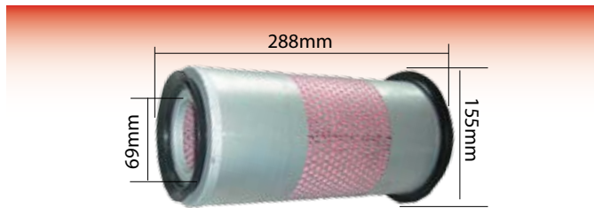
1681 Air Filter IHC 885XL Without Hole Also Hymac 370, 370C
