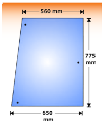
404732 Glass Overwing Left Hand Curved OE Ref: 82009813
