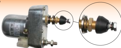
Wiper Motor Case 12V 135 Small Tapered Shaft Shaft Length 34mm
