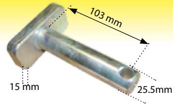
Bottom Fork Lift Link Pin CBM Type 25.50mm
