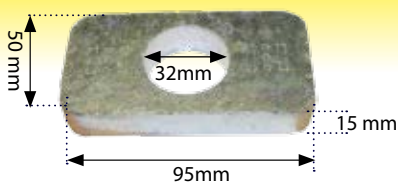
Bottom Fork Plate CBM Type 32mm hole
