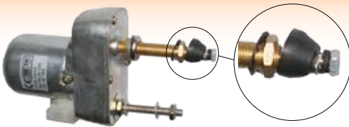
Wiper Motor 12 Volt 80 Small Tapered Shaft Shaft Length 58mm - Check Type of Cab
