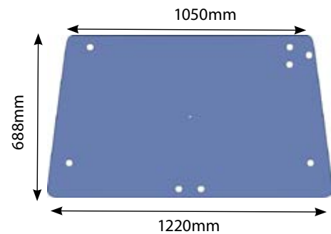
2380 Glass Case 1394 Rear Upper 8 Hole Case IHC 1190 - 1694 OE Ref: K312000
