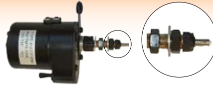
Wiper Motor 12 Volt 110 Short Stem Straight Shaft Length 46mm Arm ref is 4296
