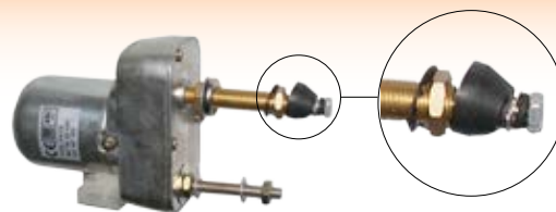
Wiper Motor 12 Volt 110 Small Tapered Shaft Shaft Length 58mm
