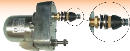
Wiper Motor Case 12V 115 Small Tapered Shaft Shaft Length 34mm
