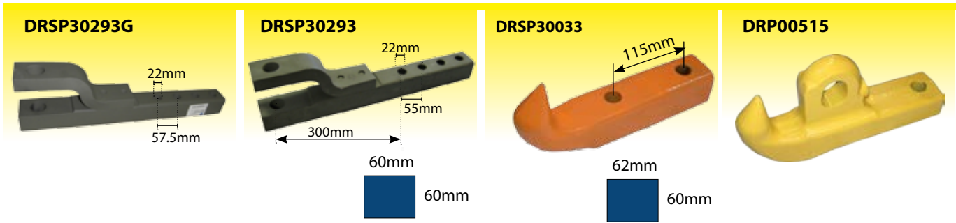
DRSP30293G Drawbar Assembly ISO 57.5mm centre to centre
