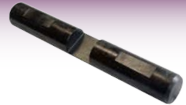
58995 Shaft Differential Bevel Gear John Deere 1530 1830 2030 2130 940 1040 1140 1640 1840 2040 2140 3040 3140 3640 3050 3350 2650 2850 2250 OE Ref: L29226
