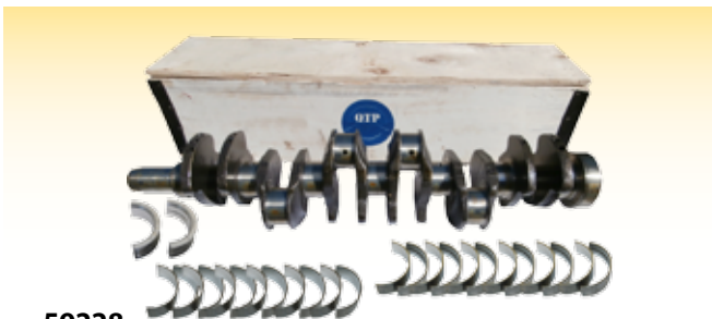
59228 Crankshaft John Deere 6 Cyl Taper Nose 6510 6910 6520 6920 6530 6930 7430 7530 OE Ref: RE505921
