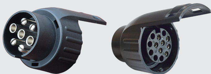
PLASTIC SOCKET 13 PIN TO 7 PIN 53912 | OE Ref: S.31357
