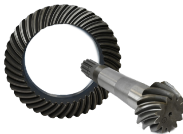
CROWN WHEEL PINION SET 400020 | OE Ref: 5128816 Fiat 90 Series
