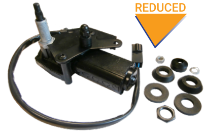
QTP DEVELOPED WIPER MOTOR FRONT 63240 | OE Ref: 3812438M91 Massey Ferguson 54s 42s 43s Series Wiper Motor fitted on Dash
