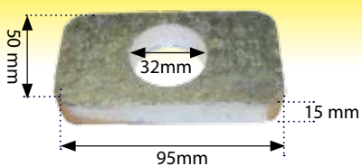
Bottom Fork Plate CBM Type 32mm hole
