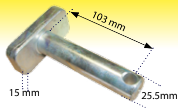
Bottom Fork Lift Link Pin CBM Type 25.50mm
