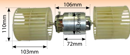
Fan Cab Blower 3000 6100 5400 6200 8100 Also fits 8200
