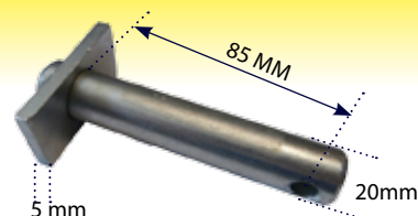
Lower Levelling Box Pin John Deere 6000
