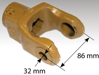
Tractor End Yoke
