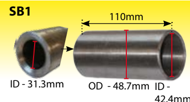
Bush Tapered Stonefork Tine 110 mm Long 48.7 mm OD 42.4 + 31.3 mm ID 19.05mm
