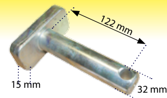
Bottom Fork Lift Link Pin CBM Type 32mm
