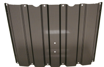
FRONT GRILL MIDDLE UPPER 59101 59102 LOWER / 59103 LH / 59104 RH John Deere 6520 6620 6820 6920 6530 6630 6830 6930 Series
