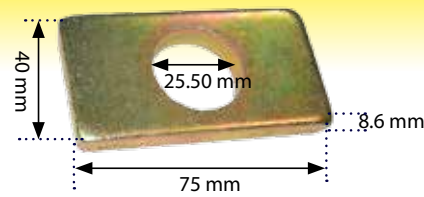
Fork Plate John Deere 76 77 7810 Bottom
