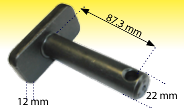
Bottom Fork Lift Link Pin CBM Type 22mm
