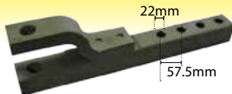
Drawbar Assembly ISO
